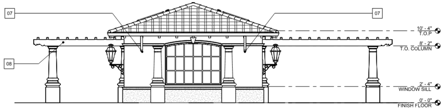
42 NORTH ELEVATION 1/4" = 1'-0"
